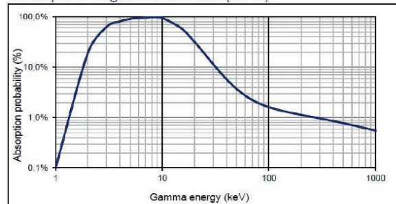
Absorption of gamma radiation (23 °C)
