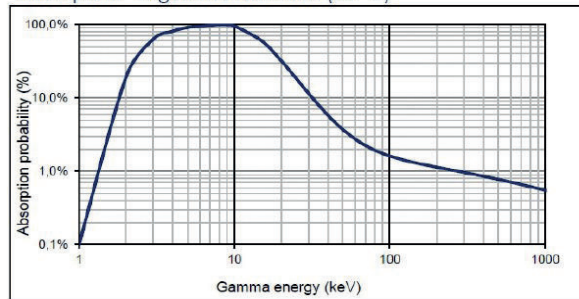
Absorption of gamma radiation (23 °C)
