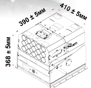
LA-ML15 Grenade Launcher with optional colored night vision
