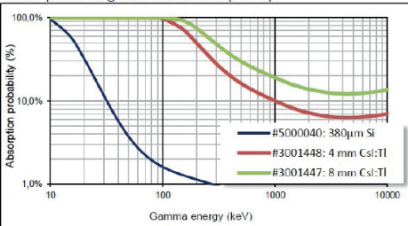
Absorption of gamma radiation (23 °C)
